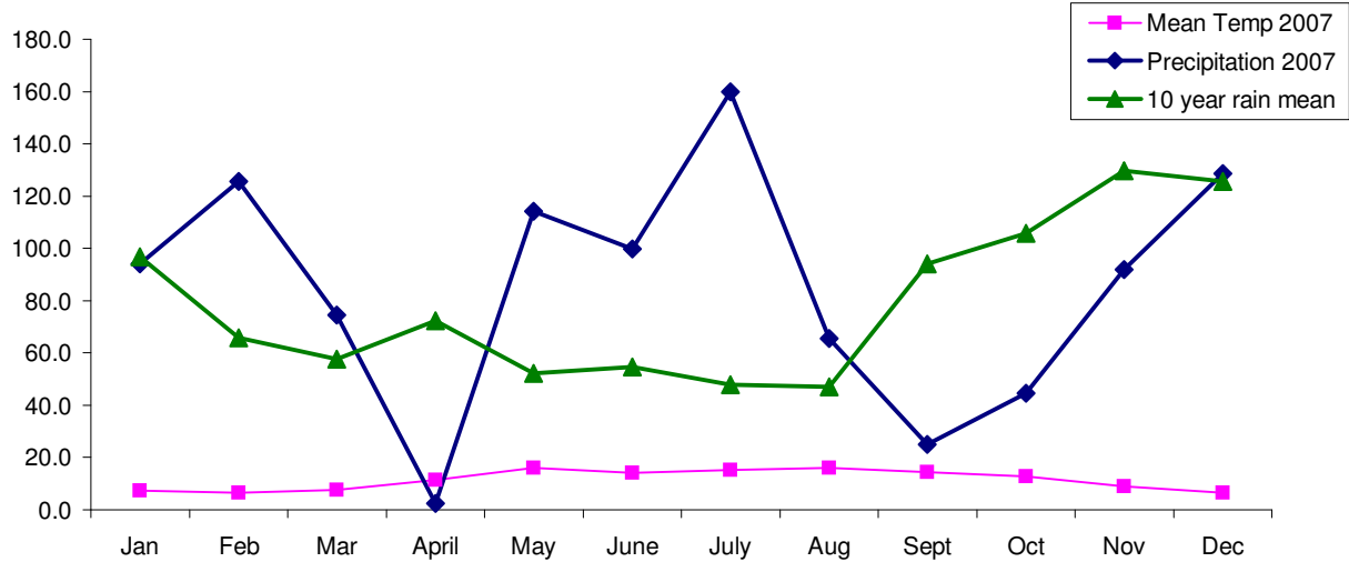
2007 monthly Rainfall (compared with 10 year mean rainfall)
