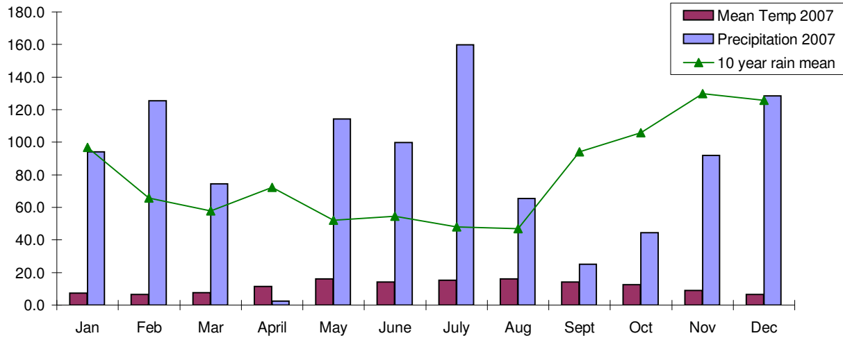
2007 mean Temperature and Rainfall (compared with 10 year mean rainfall)
