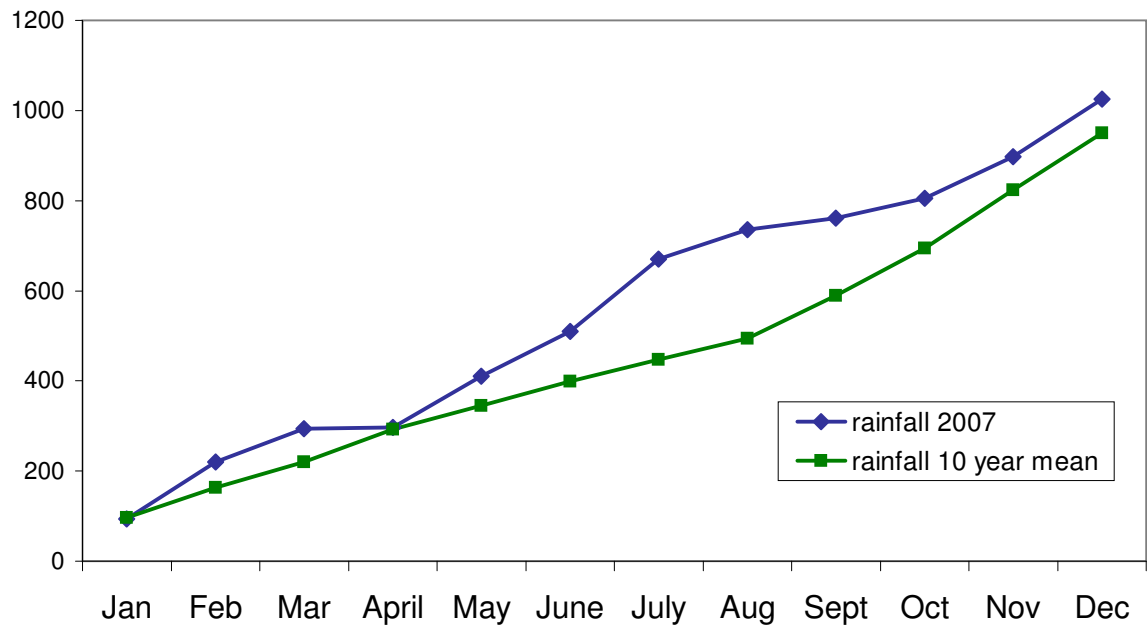
Cumulative Monthly Rainfall 2007 cf 10 year mean
